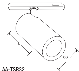
AA-TSR32 (OD) 78mm Overall (Ø) (L) 100mm Length
